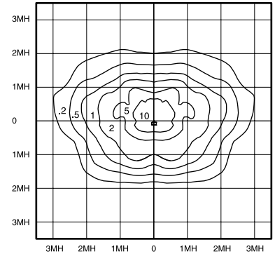
175 Watt Metal Halide, 0°
