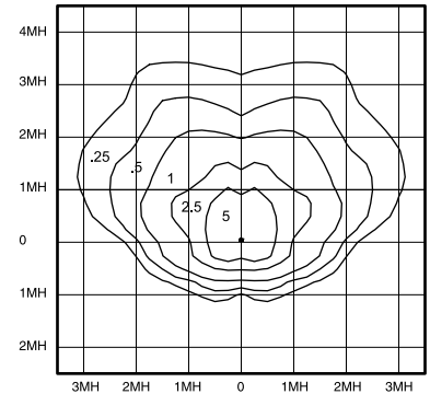
175 Watt Metal Halide, 22.5°
